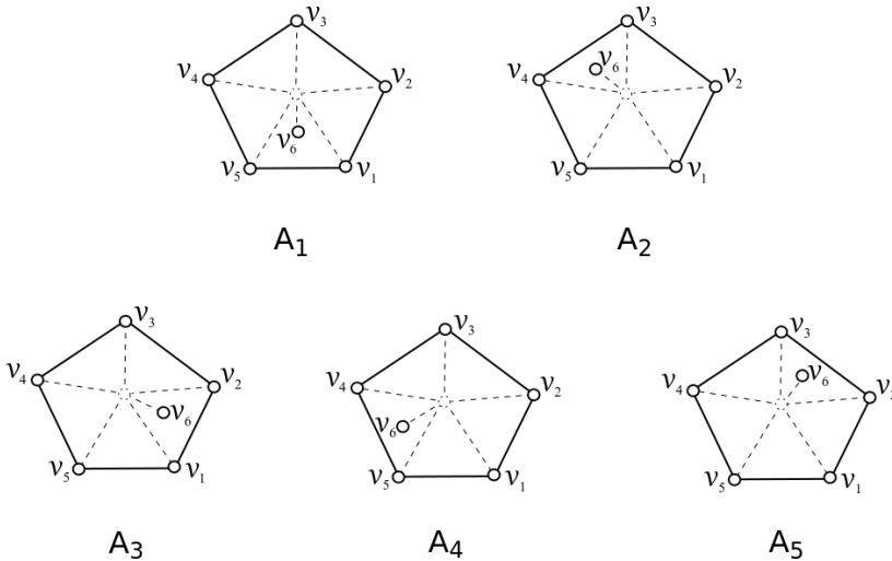
FIGURE 2. Drawings of five possible configurations of the subgraph F^i.
