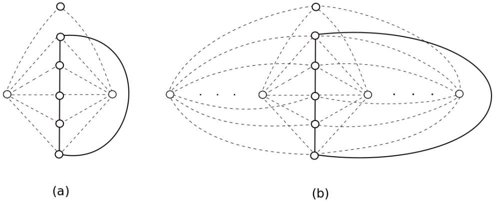
FIGURE 3. The good drawings of G + D_2 and of G + D_n .
