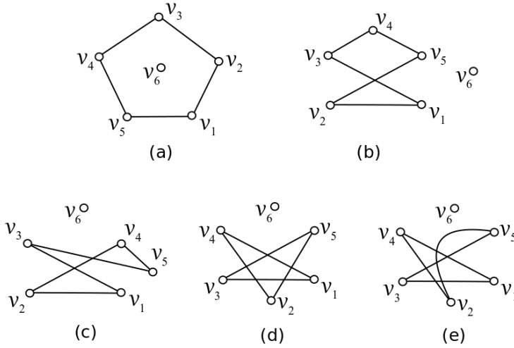
FIGURE 1. Five possible drawings of the graph G .
