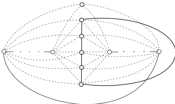
FIGURE 5. The good drawing of G + P_n with 6 \lfloor \frac{n}{2} \rfloor \lfloor \frac{n-1}{2} \rfloor + \lfloor \frac{n}{2} \rfloor + 1 crossings.
