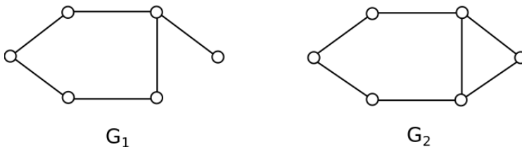
FIGURE 4. Two graphs G_1 and G_2 by adding new edges to the graph G .
